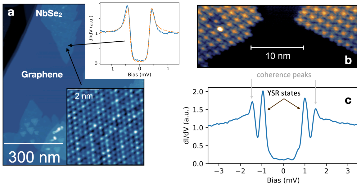
Figure 1 : (a) STM topograph of submonolayer MBE-grown NbSe 2 on graphene. The insets show an atomically resolved zoom and a tunneling spectroscopy of the NbSe 2 . The orange dashed line is a fit. (b) Self-assembled monolayer of MnPc molecules on the Pb(111) surface. (c) Tunneling spectroscopy of a magnetic bound state on an individual MnPc molecule in (b), displaying the superconducting bound states. All data taken at 50 mK.
